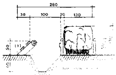
Open-ditch
