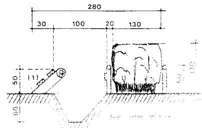
Open-ditch
